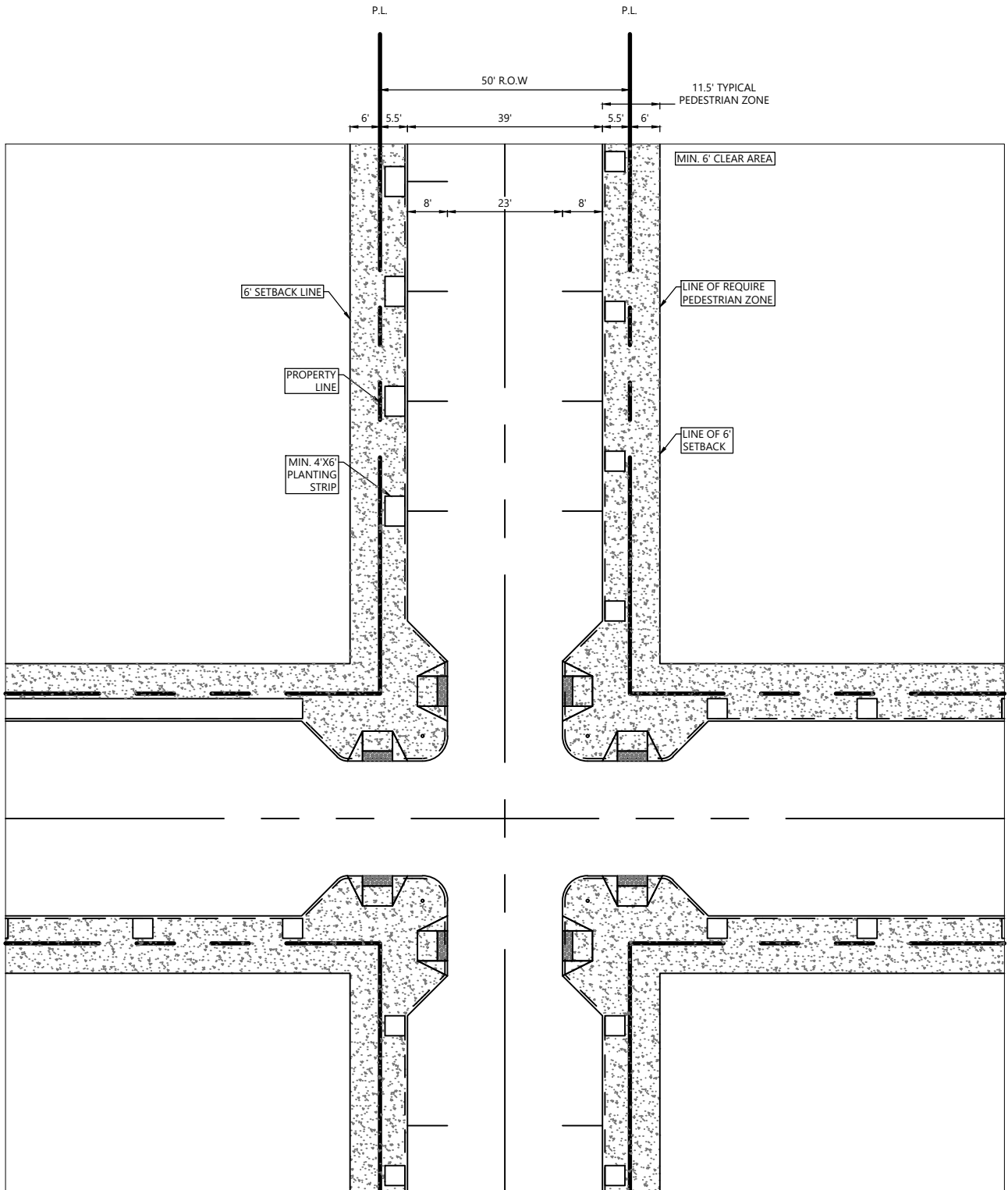
50' R.O.W. @ SUBDISTRICT 1E PLANTING STRIP
